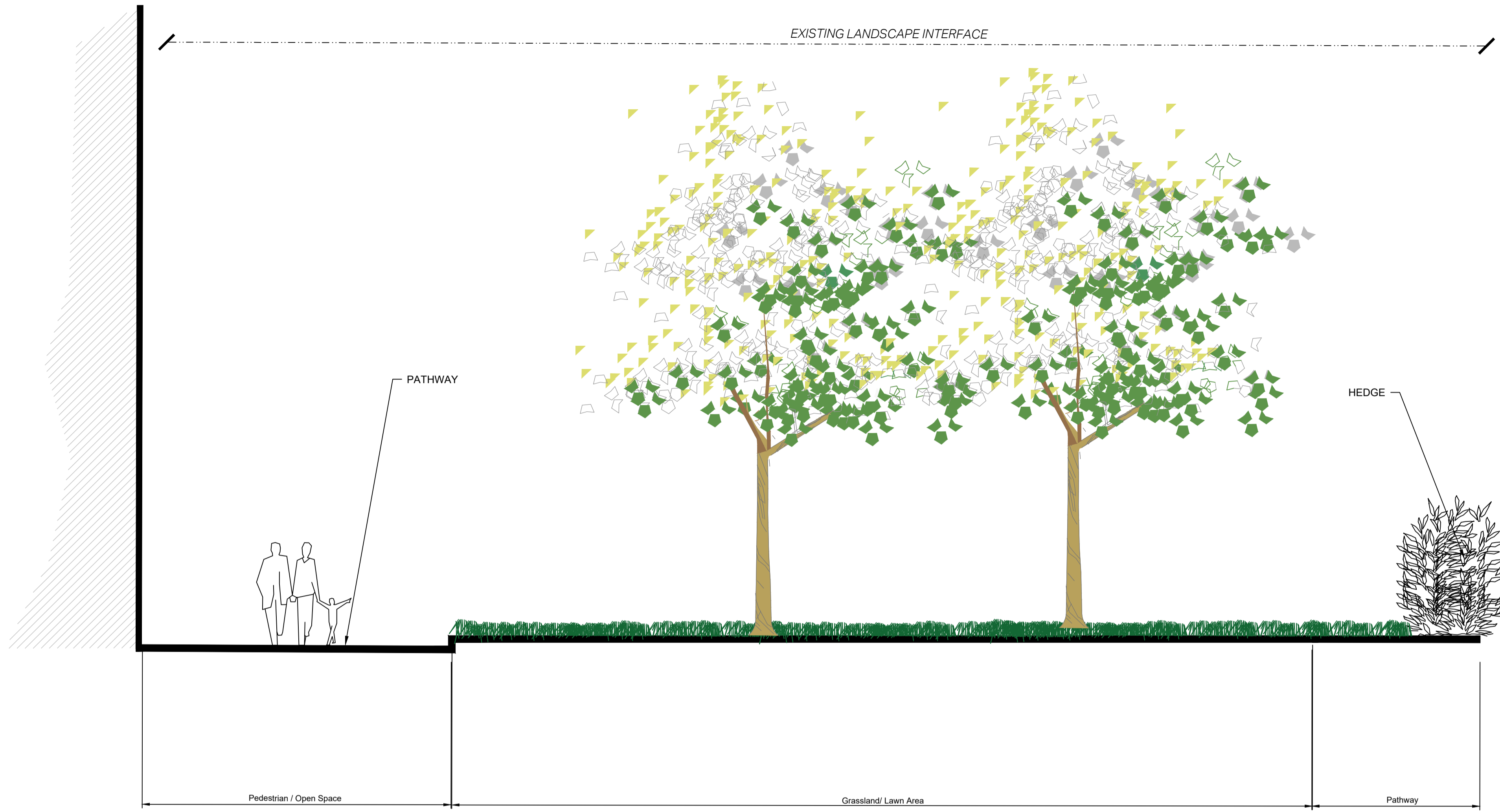
12 INTERFACE BETWEEN EXISTING LANDSCAPE AND THE BUILDING L-L SCALE: 1:50
